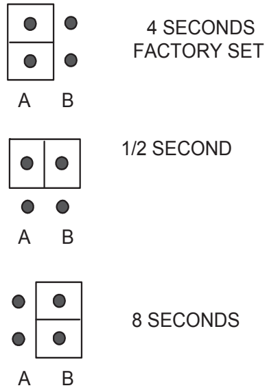
Diagram 16 Time Set Jumper
