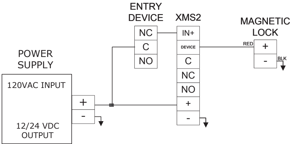
Diagram 11 Wiring with Entry Device
