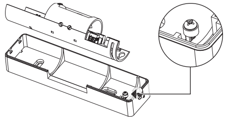
Diagram 6 Back Bracket
