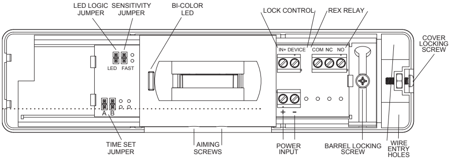
Diagram 9 XMS2 Overview
