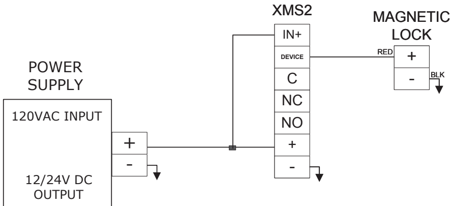
Diagram 10 Wiring Magnetic Lock Only
